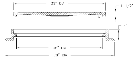
Available Frames for 1475 Covers and Grates
